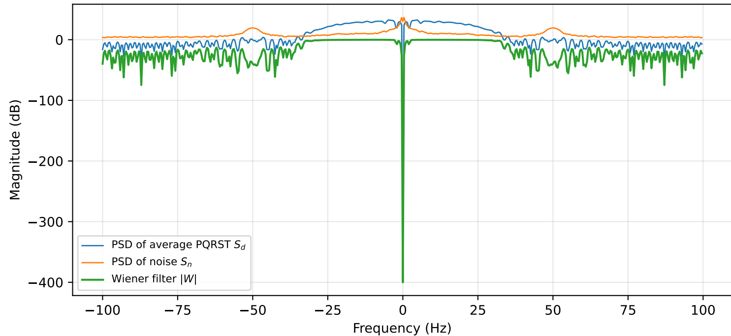
Desired-signal PSD, noise PSD and Wiener transfer function
